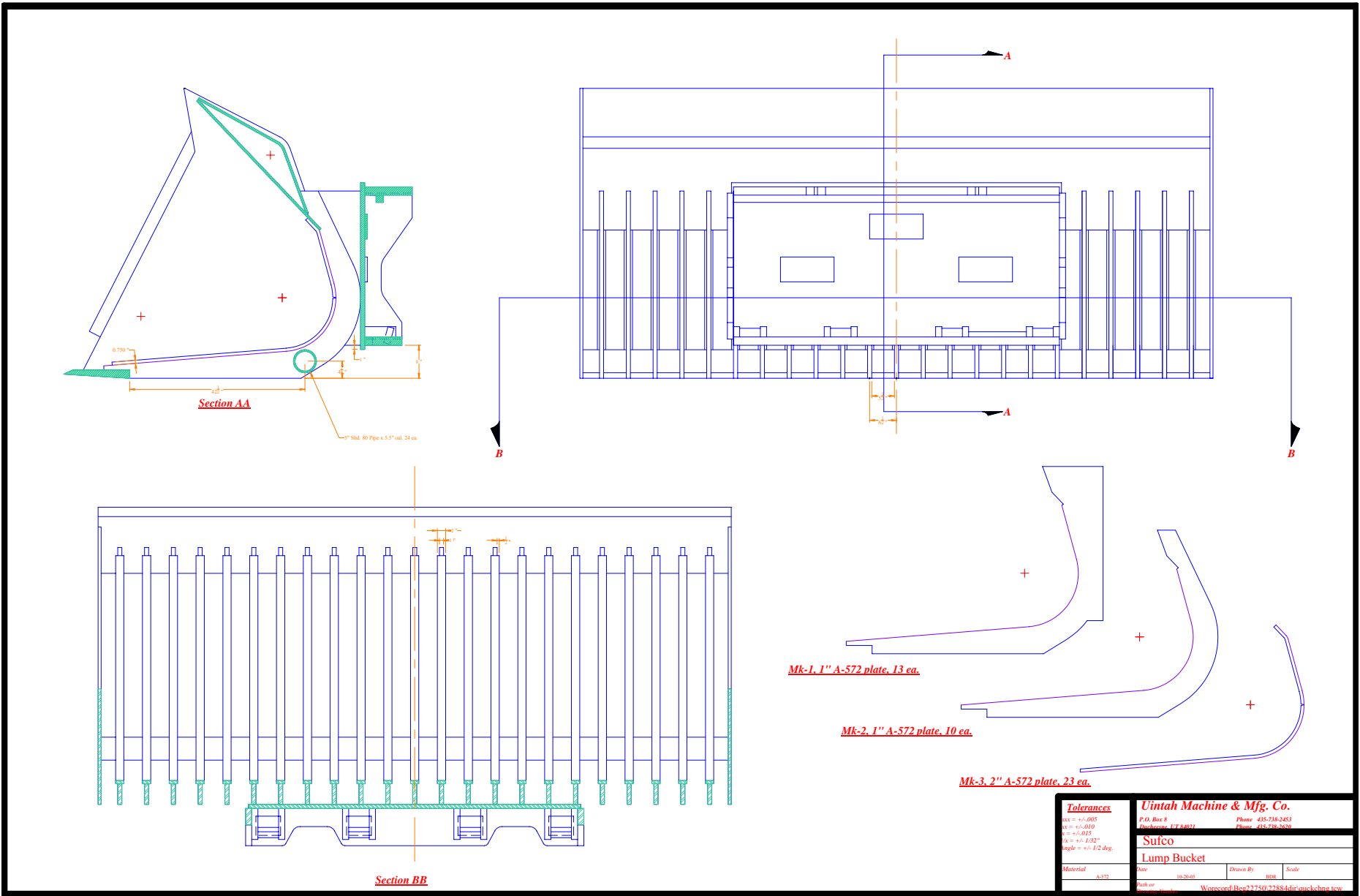
Lump bucket with quick-change feature for sorting coal in a front-end loader.
