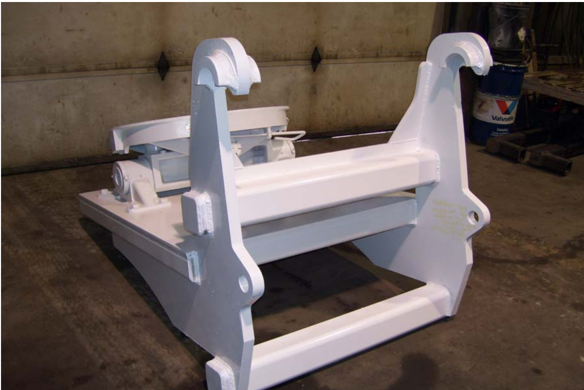
FIFTH WHEEL ATTACHMENT FOR QUICK COUPLER
